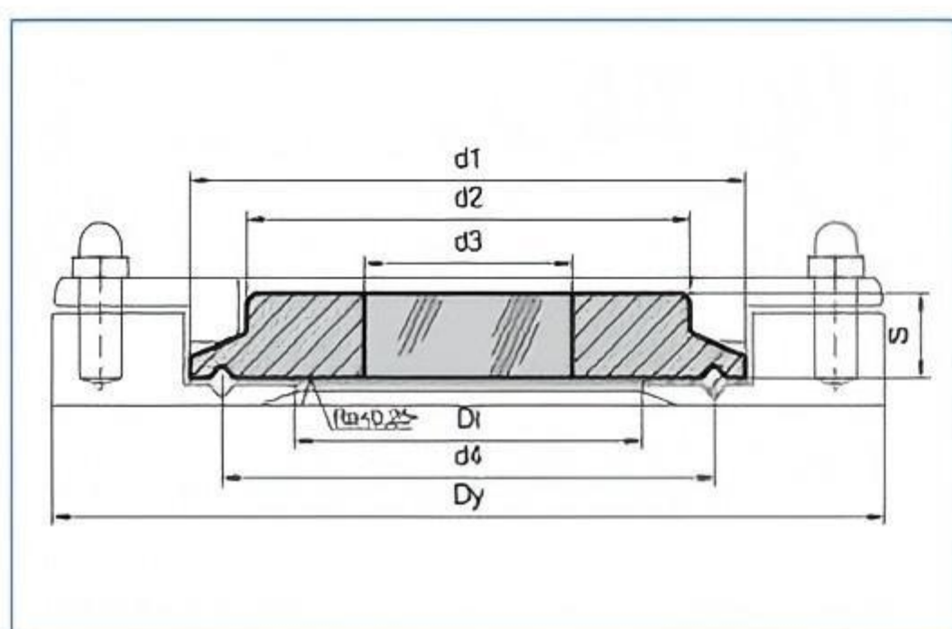
Typical assembly
