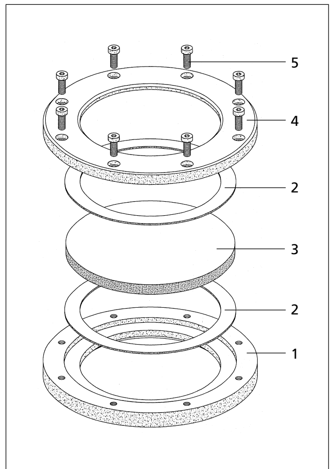
Structure of a Lumiglas sight glass fitting made of stainless steel
