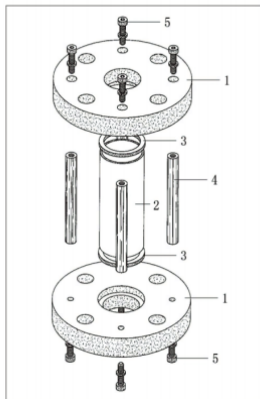
Schematic diagram of the structure of the flow sight glass
